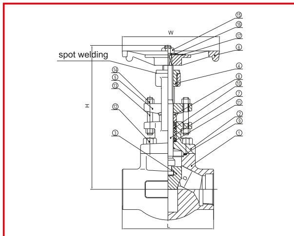
Bolted Bonnet
