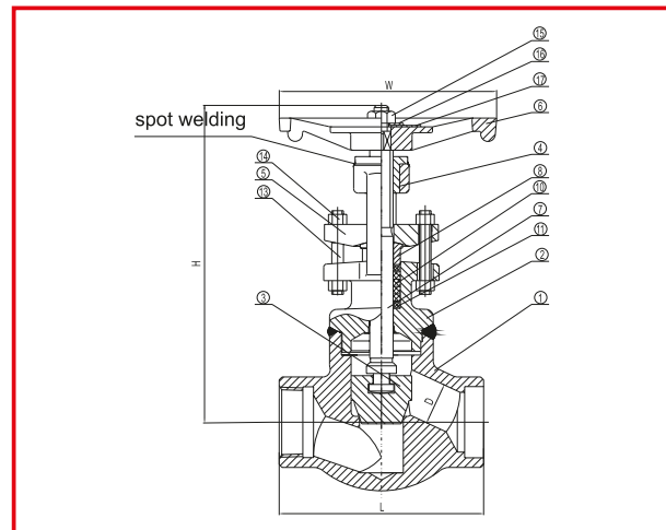
Welded Bonnet
