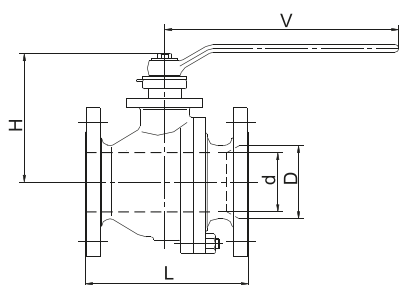
Adapta Class 150, Class 300LB.BM Series
