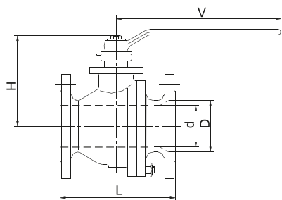
Adapta Class 150、Class 300.BM Series
