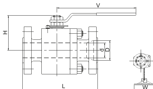
Adapta Class 600.BM Series
