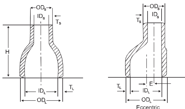
REDUCER
