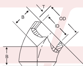
45° ELBOWS
