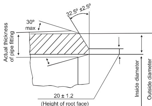
Fig.2 Shape and dimensions of bevel end
