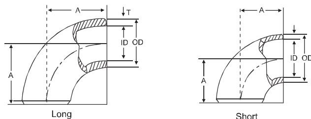
90° ELBOWS
